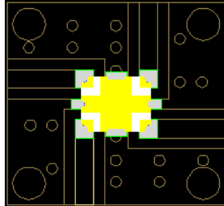
Figure 11. Placing the RCP2150Q10 on the 9 Points of the PCB Surface
