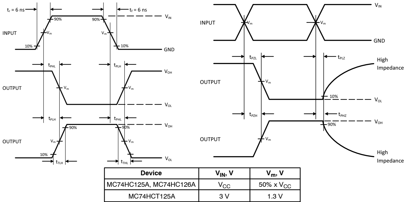
Figure 4. Switching Waveforms
