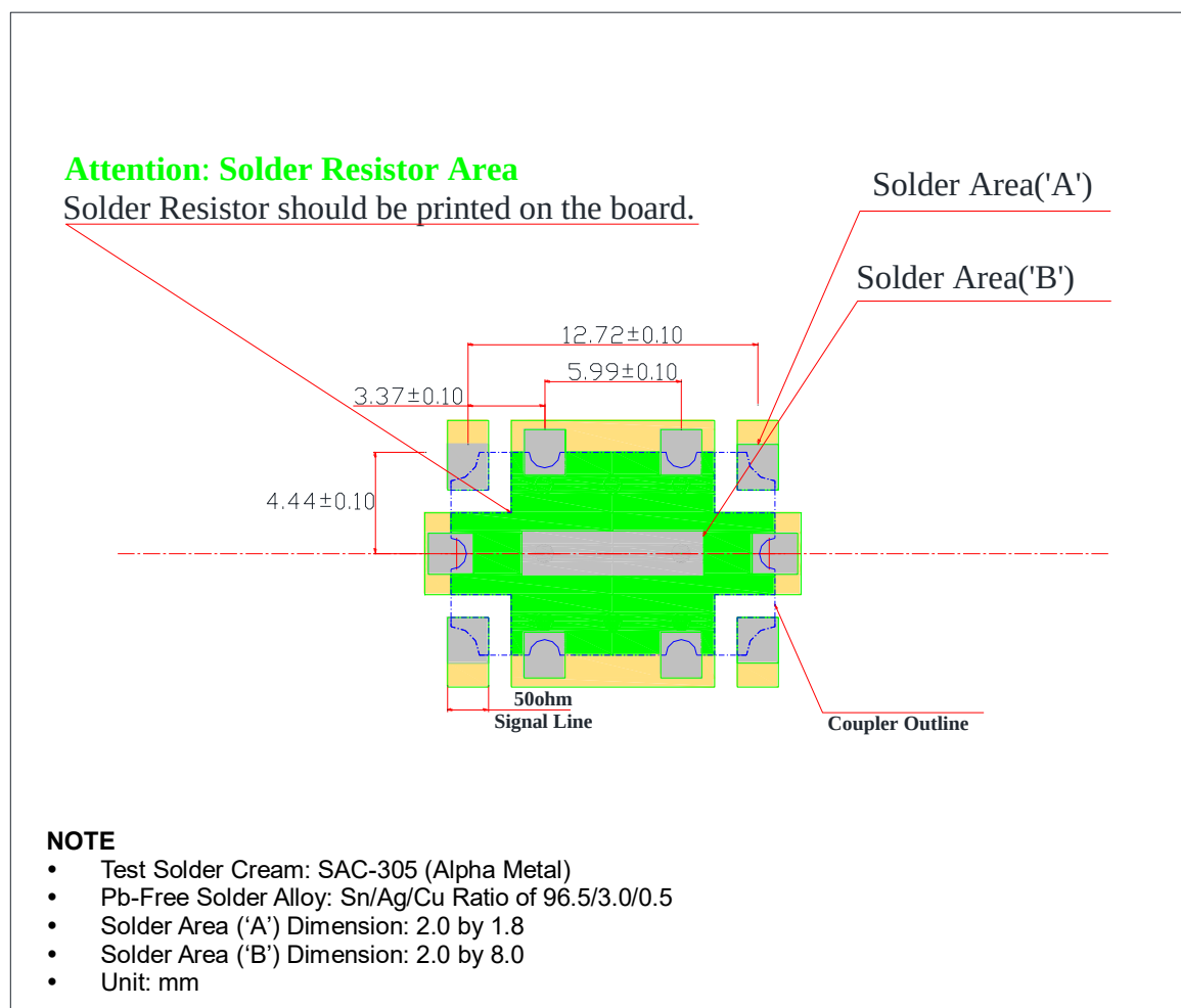
Figure 8. Recommended PCB Layout and Solder Mask Pattern
