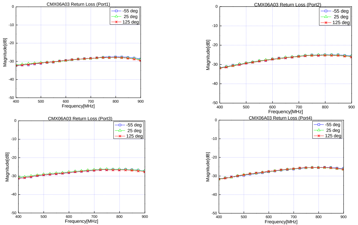
Figure 3. Test Plots of Return Loss (-55 °C, 25 °C and 125 °C)
