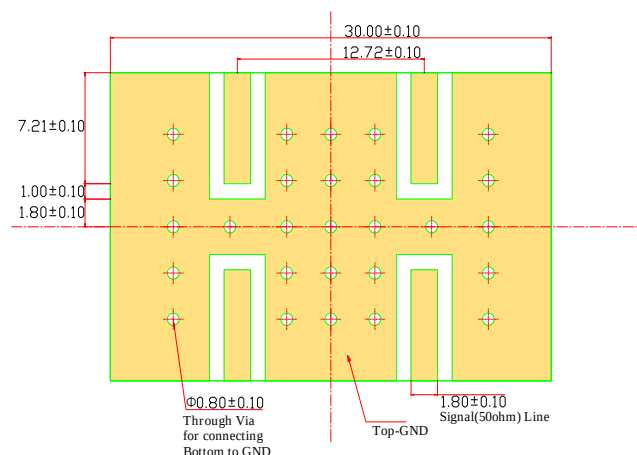
Figure 6. RN2 Technologies Test Board Layout
