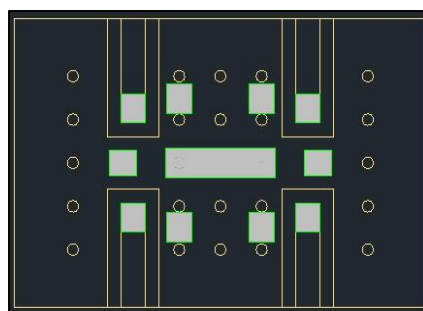
Figure 10. Applying the Solder Paste to the 11 Points on the PCB Surface
