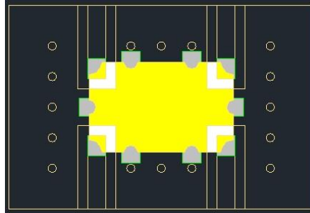
Figure 11. Placing the CMX06A03 on the 11 Points of the PCB Surface
