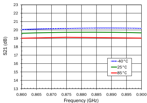
S21 versus Frequency
