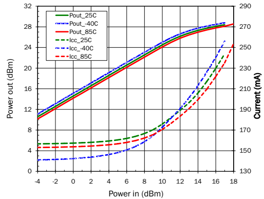
Power out & Current versus Pin @ 2140MHz
