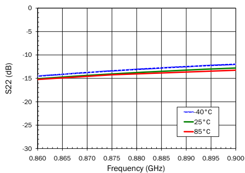
S22 versus Frequency
