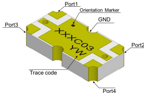
Figure 1. RCP2250C03 (Top View)
