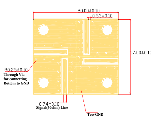
Figure 6. RN2 Test Board Layout
