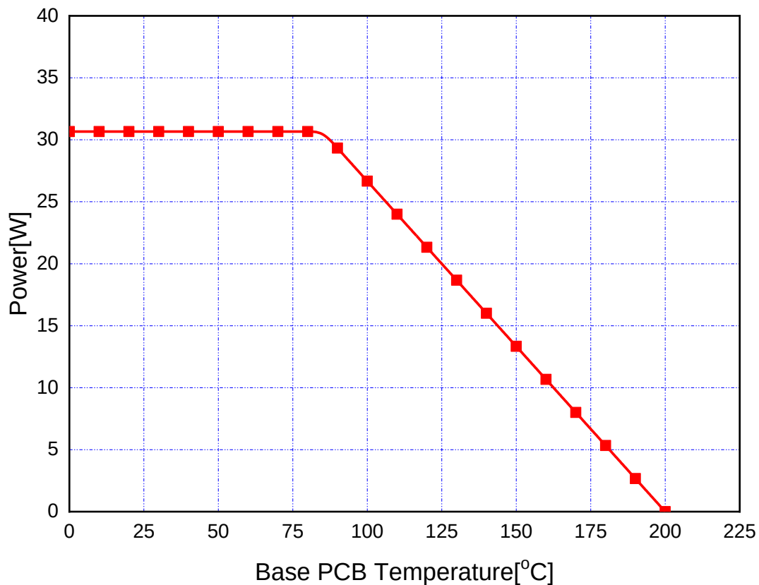
Figure 2. Power Derating Curve
