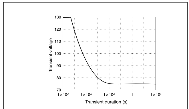
Single voltage pulse at +25°C ambient temperature.
