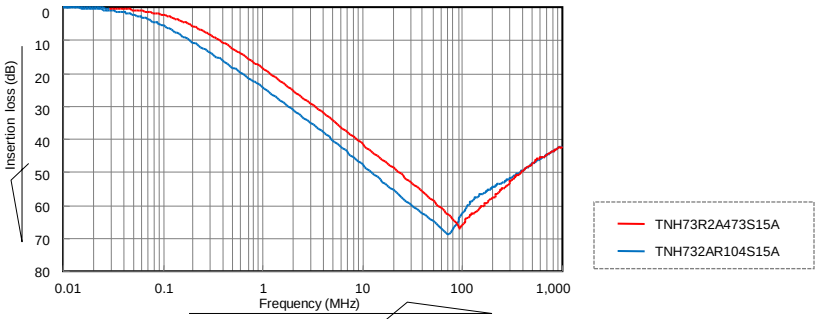
Insertion Loss Characteristics (Reference)
