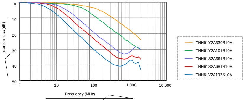
Insertion Loss Characteristics (Reference)
