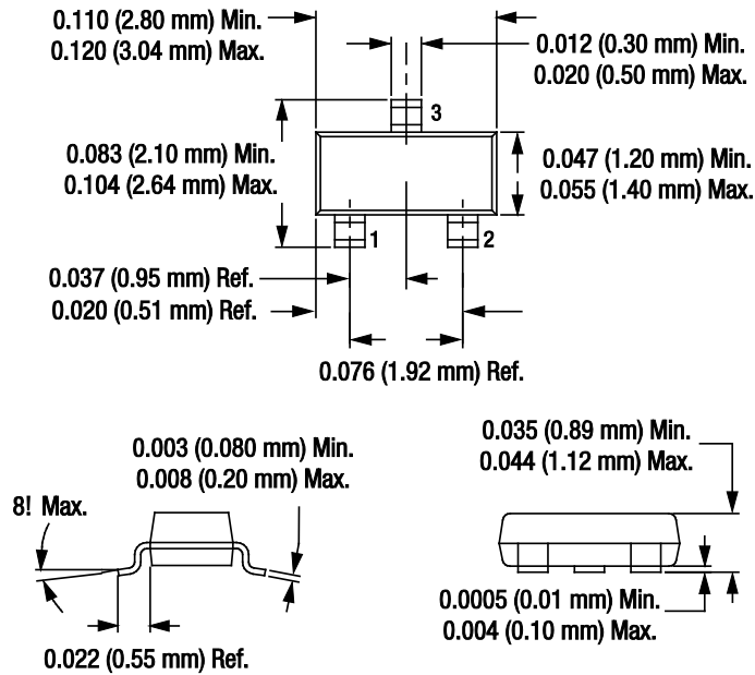
Figure 14. SOT-23 Package Dimensions
