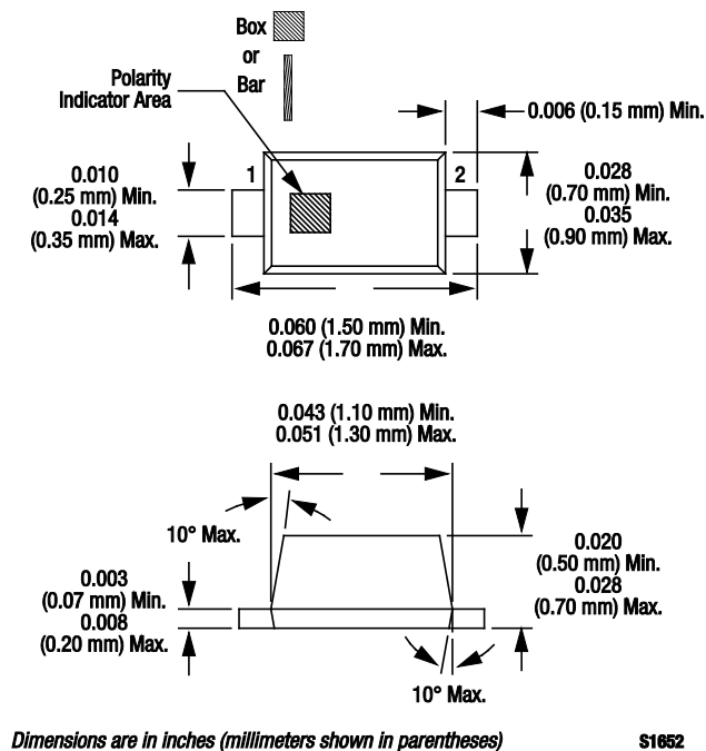
Figure 8. SC-79 Package Dimensions
