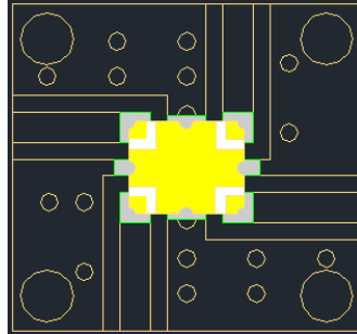
Figure 11. Placing the CMX07Q03 on the 9 Points of the PCB Surface
