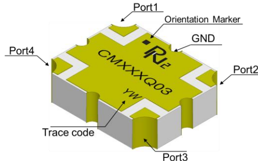
Figure 1. CMX07Q03 (Top View)
