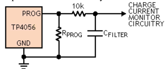
Fig.2 Isolating Capacitive Load on PROG Pin and Filtering
