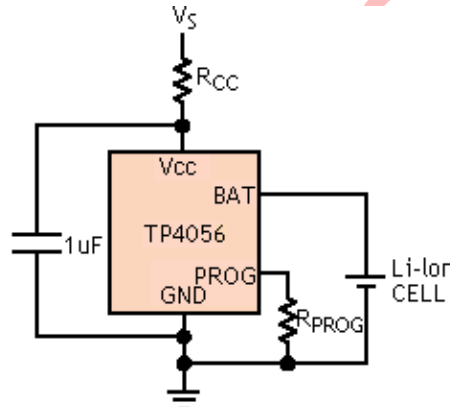
Fig.3 Circuit Example to Increase Charging Current
