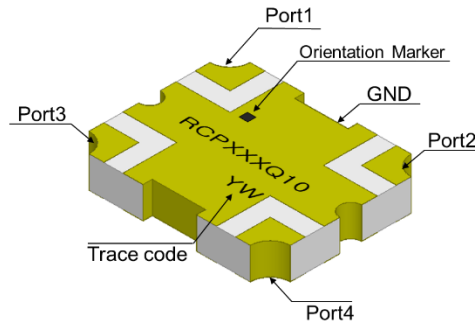
Figure 1. RCP2650Q10 (Top View)
