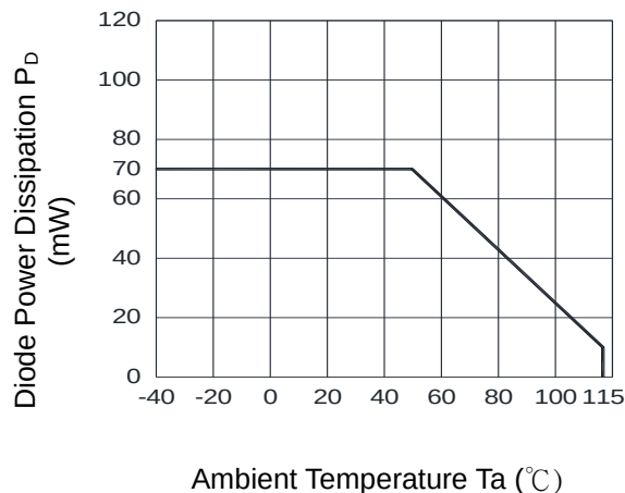
Fig.2 Diode Power Dissipation vs. Ambient Temperature
