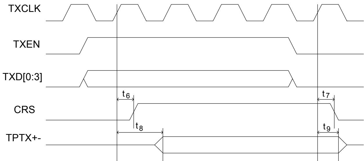
Figure 18. MII Transmission Cycle Timing-2
