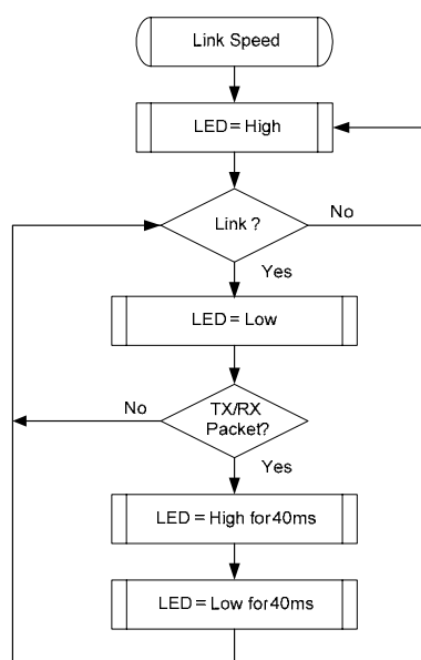
Figure 10. LINK/ACT LED
