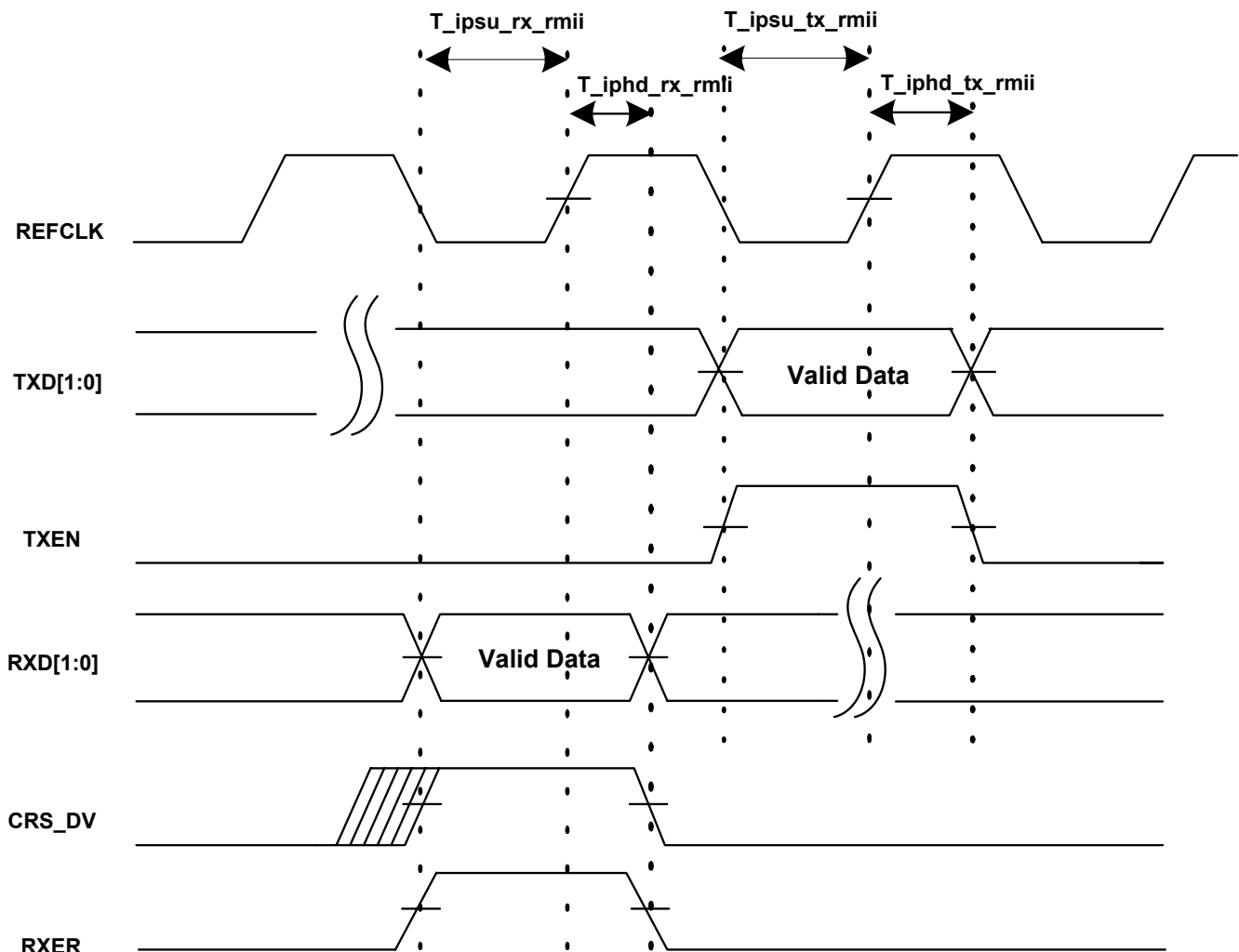
Figure 21. RMII Transmission and Reception Cycle Timing
