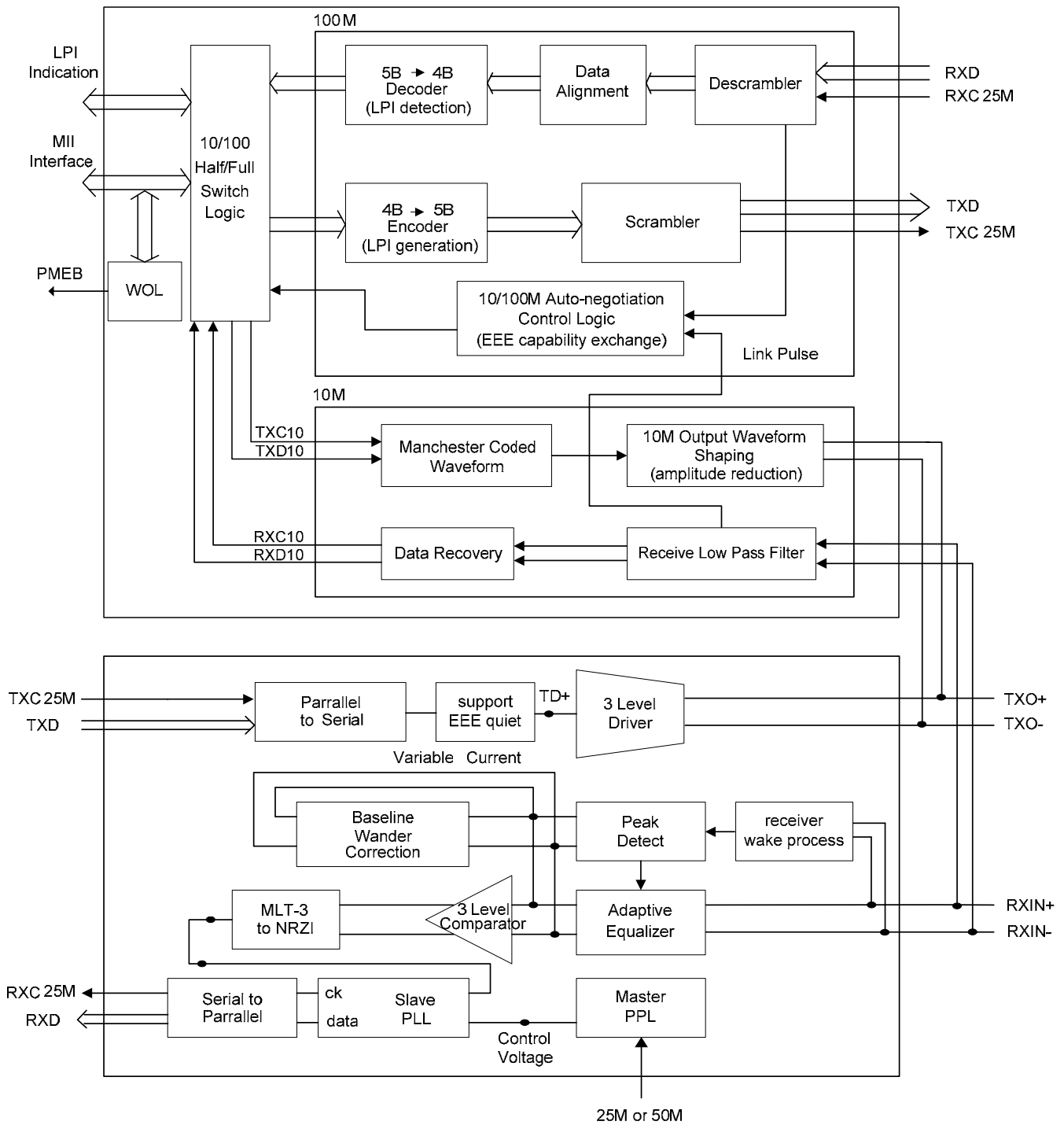
Figure 1. Block Diagram
