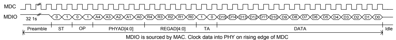
Figure 6. Write Cycle
