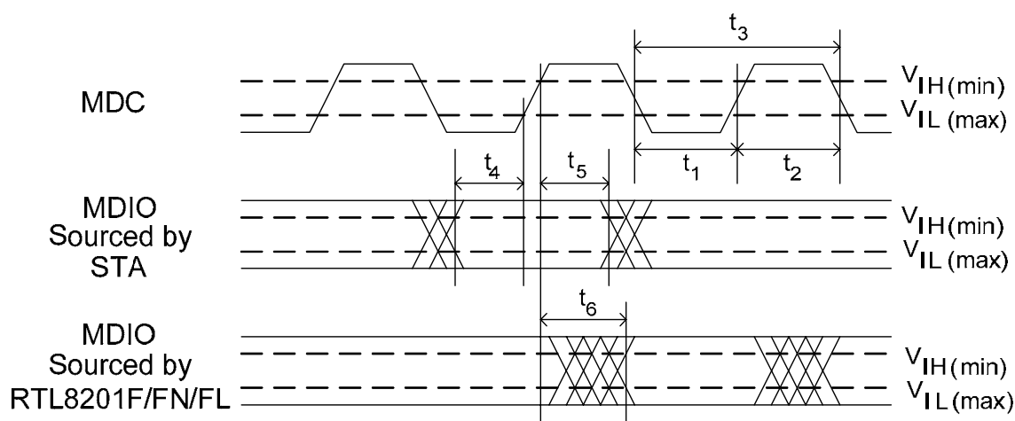
Figure 22. MDC/MDIO Timing
