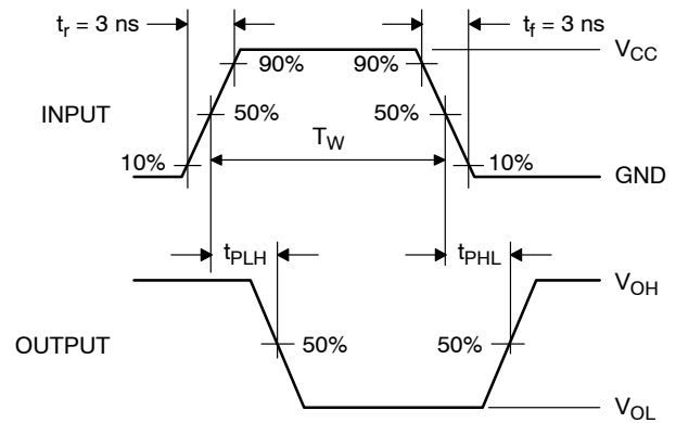
Figure 6. AC Waveforms
