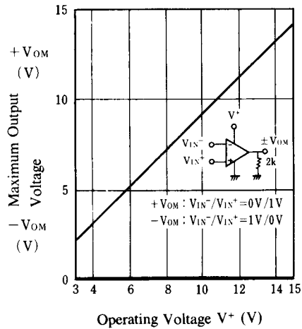
Maximum Output Voltage vs. Operating Voltage
