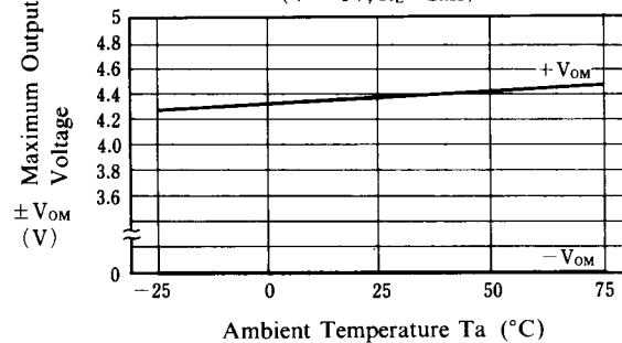
Maximum Output Voltage vs. Temperature
