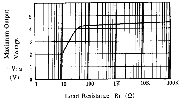
Maximum Output Voltage vs. Load Resistance
