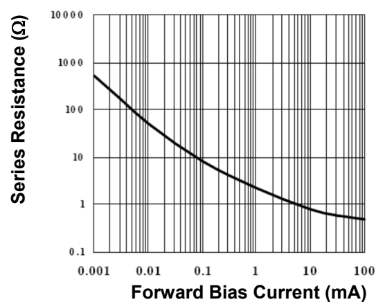
Resistance vs. Forward Current (MADP-007448 Series)
