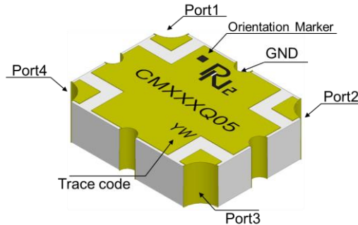
Figure 1. CMX09Q05 (Top View)
