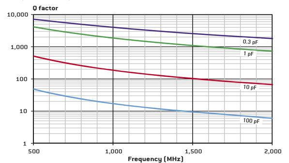
SHF (SIZE 0805): TYPICAL Q FACTOR VERSUS FREQUENCY
