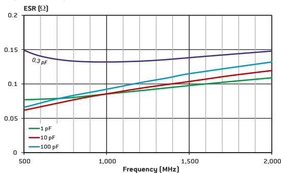
SHL (SIZE 0402): TYPICAL ESR VERSUS FREQUENCY
