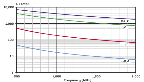
SHL (SIZE 0402): TYPICAL Q FACTOR VERSUS FREQUENCY
