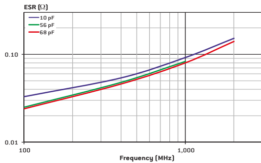
SHS (SIZE 0603): TYPICAL ESR VERSUS FREQUENCY
