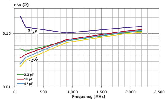
SHF (SIZE 0805): TYPICAL ESR VERSUS FREQUENCY
