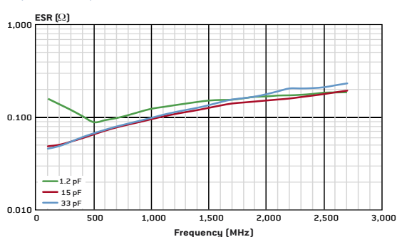
SHL (SIZE 0402): TYPICAL ESR VERSUS FREQUENCY
