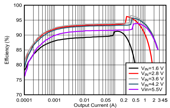
Efficiency Target vs Output Current ( V_{OUT} = 3.3 V)
