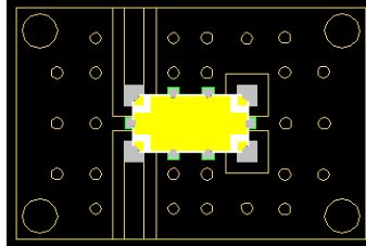
Figure 10. Placing the DL2 on the 11 Points of the PCB Surface
