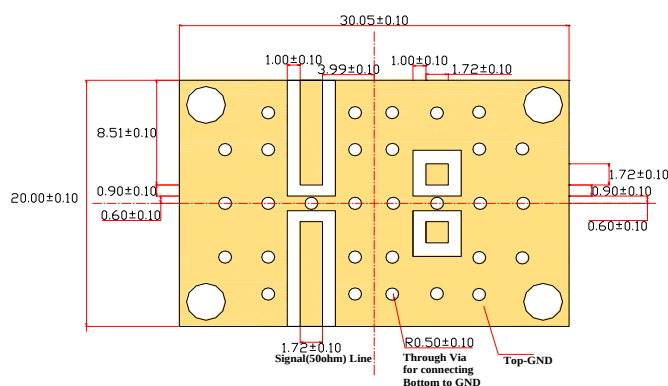
Figure 5. RN2 Technologies Test Board Layout
