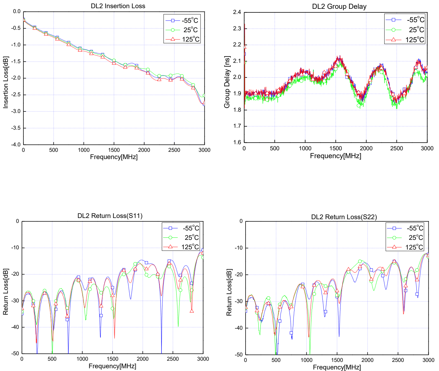
Figure 3. Test Plots of Insertion Loss, Group Delay and Return Loss (at -55 °C, 25 °C, and 125 °C)
