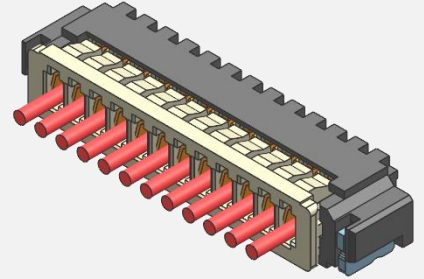
Mating View
