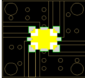
Figure 11. Placing the RCP890Q10 on the 9 Points of the PCB Surface
