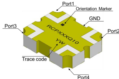
Figure 1. RCP890Q10 (Top View)
