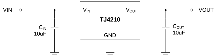
Typical 3 Pin Application
