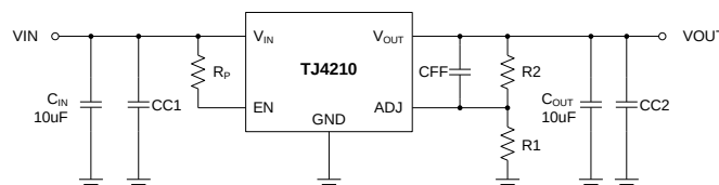
Fig. 2. Application with Feed-Forward Capacitor, CFF
