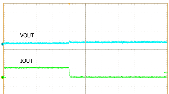
Load Transient Response (Cff=10nF, R2=51K \Omega , R1=24K \Omega )
