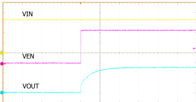
Start Up by external VEN @ Iout=0A (Cff=10nF, R2=51K \Omega , R1=24K \Omega )
