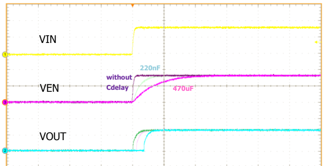
Start Up with Cdelay @ Iout=10mA (Cdelay is varied, Cff=10nF, R2=51K \Omega , R1=24K \Omega )
