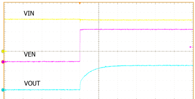
Start Up by external VEN @ Iout=1A (Cff=10nF, R2=51K \Omega , R1=24K \Omega )
