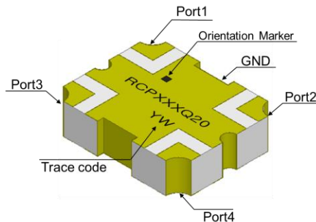
Figure 1. RCP890Q20 (Top View)
