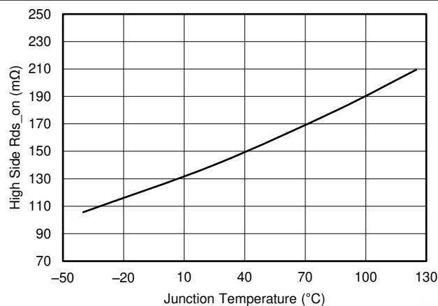
Figure 5-5. High-Side R_{ds-on} vs Junction Temperature
