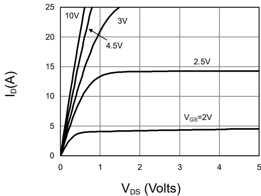
Fig 1: On-Region Characteristics
