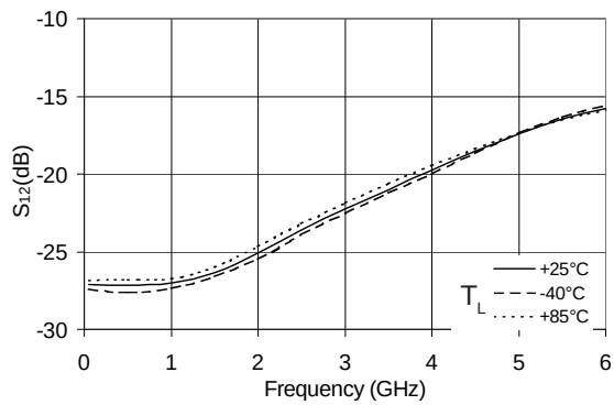
S_{12} vs. Frequency V_D = 3.9 V, I_D = 60 mA (Typ.)
