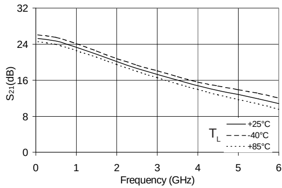
|S_{21}| vs. Frequency V_D = 3.9 V, I_D = 60 mA (Typ.)
