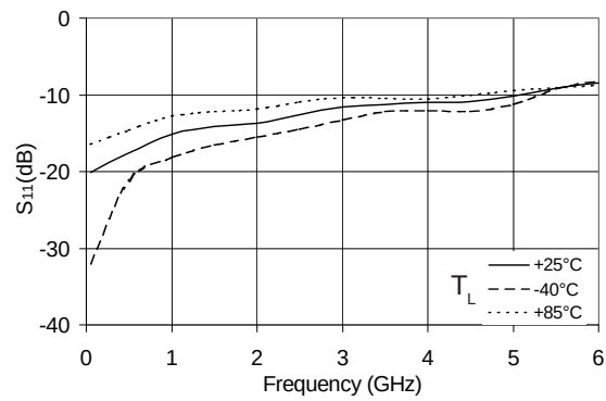
S_{11} vs. Frequency V_D = 3.9 V, I_D = 60 mA (Typ.)
