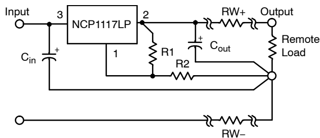
Figure 36. Load Sensing
