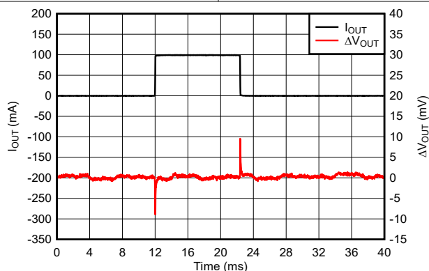
Figure 5-43. TPS76933 Load Transient Response (New Chip)
