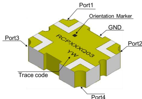
Figure 1. RCP2150Q03 (Top View)
