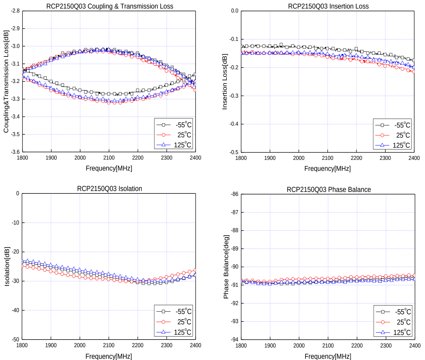
Figure 4. Test Plots of Amplitude Balance, Insertion Loss, Isolation, and Phase Balance (-55 °C, 25 °C, and 125 °C)
