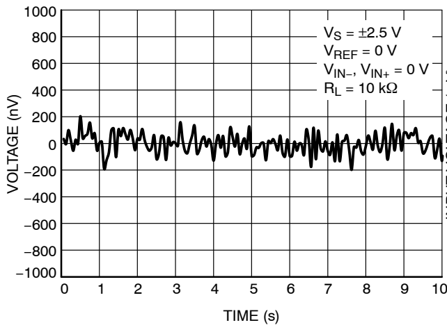
Figure 23. 0.1\text{ Hz} to 10\text{ Hz} Voltage Noise (Referred to Input)
