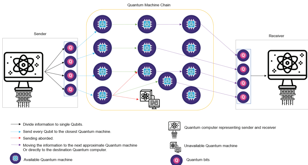
Fig. 4. Model overview of quantum machine chain.
